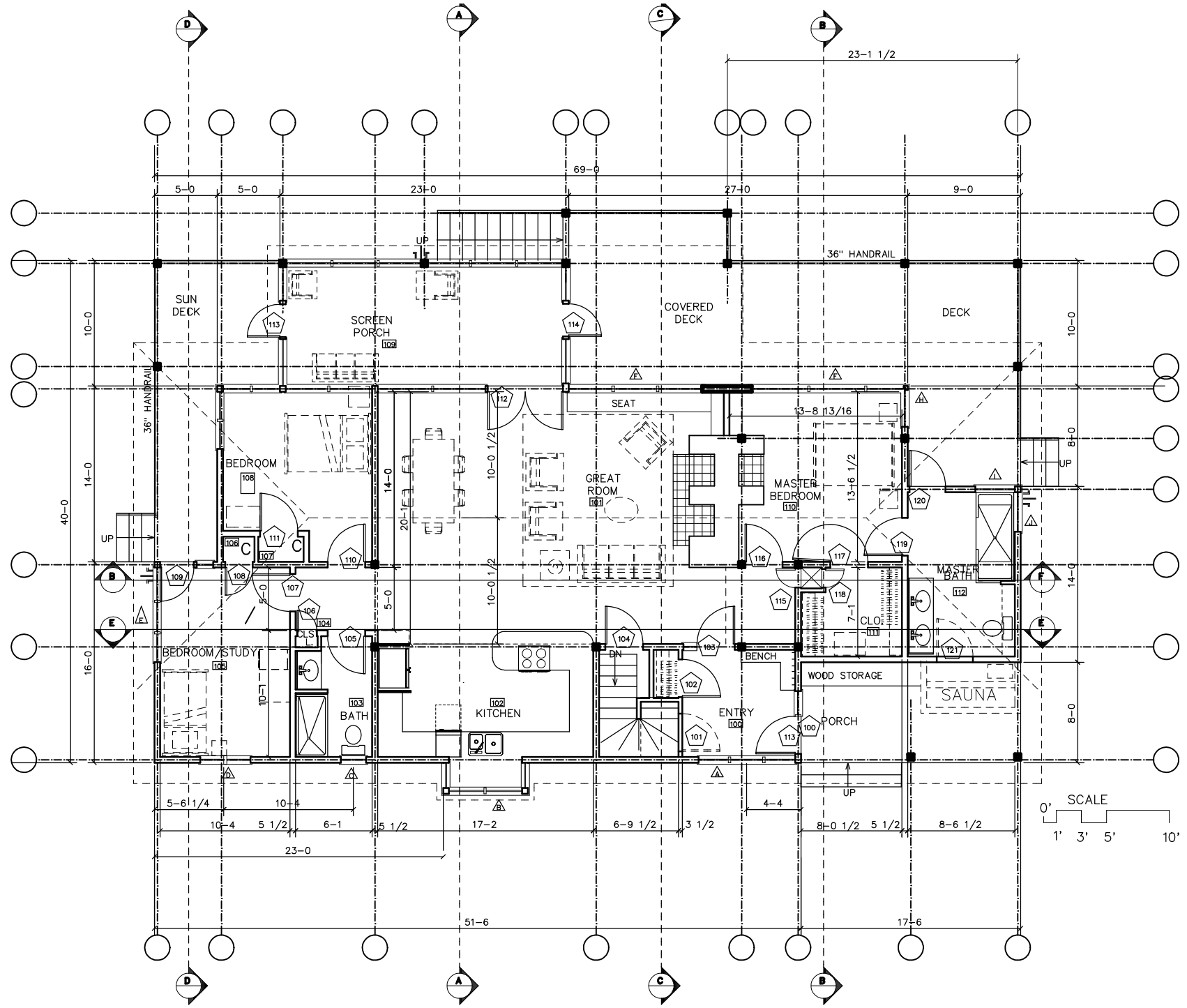
FLOOR PLAN HOUSE=2,036 ft SUN DECK=xx ft DECK=xx ft PORCH=112 ft SAUNA=32 ft
