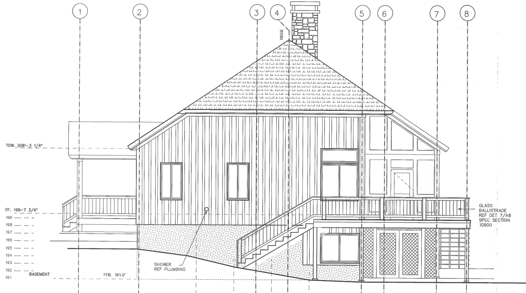
NORTH ELEVATION 1/4" = 1'-0"
