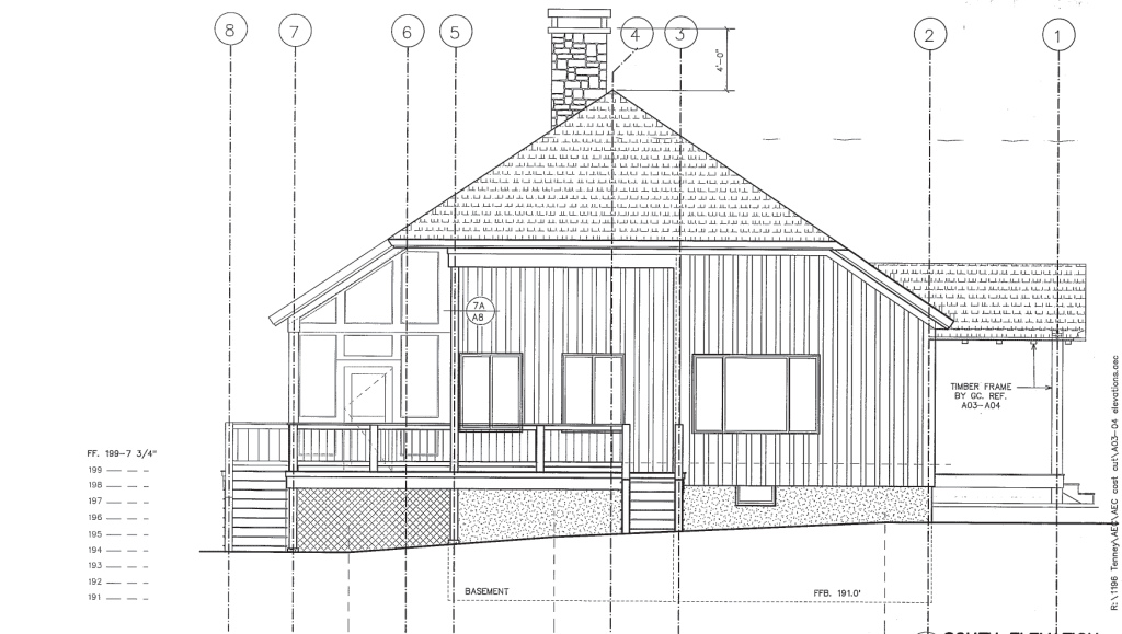
SOUTH ELEVATION 1/4" = 1'-0"
