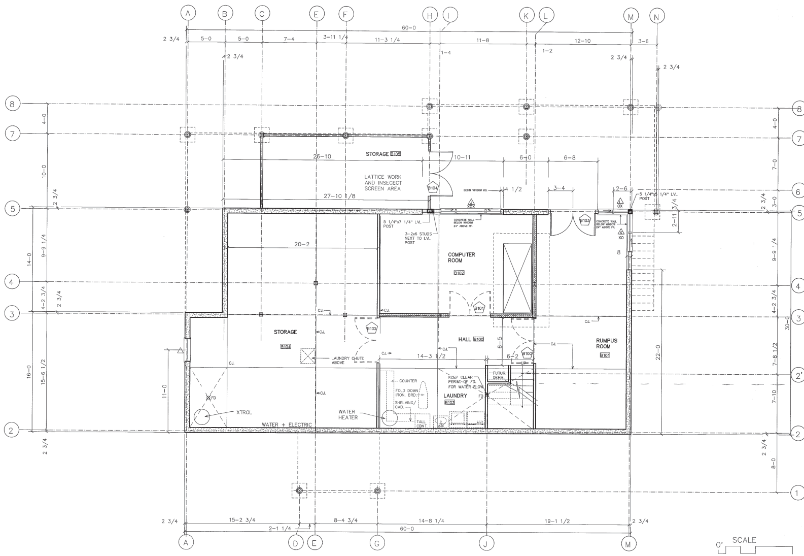
1 BASEMENT PLAN A02 1/4" = 1'-0"
